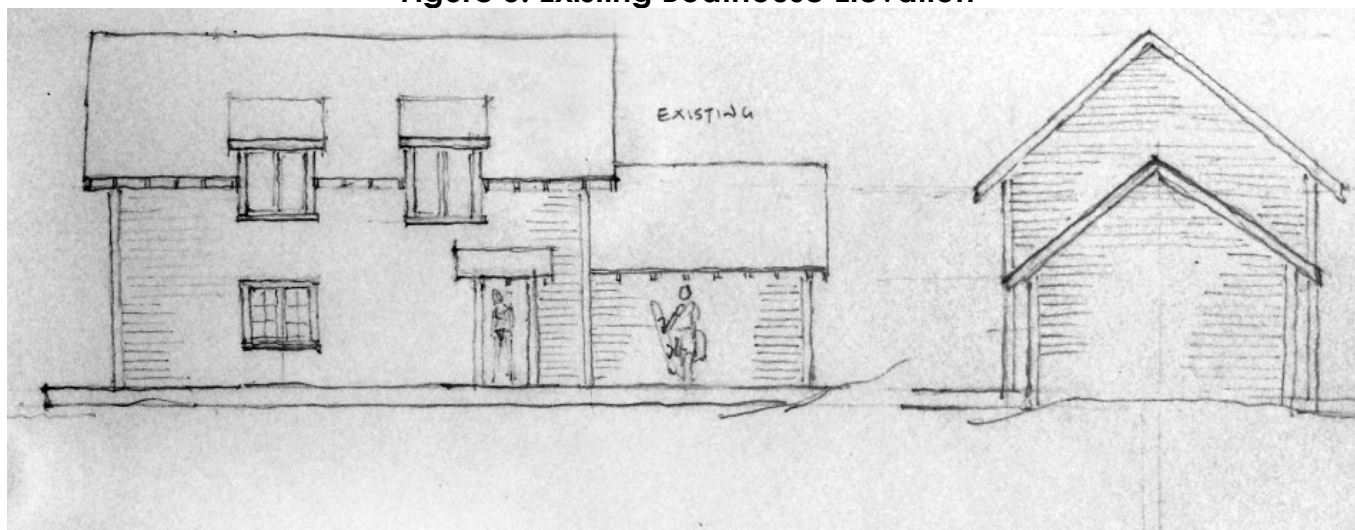
Figure 5: Existing Boathouse Elevation
