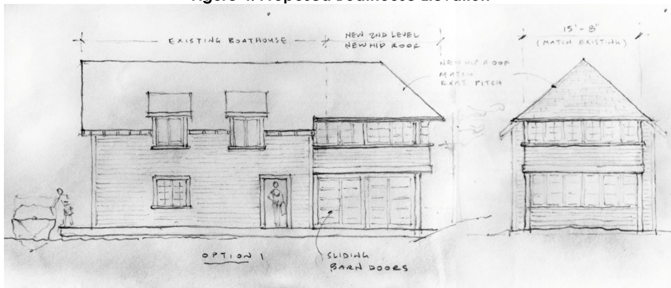
Figure 4: Proposed Boathouse Elevation
