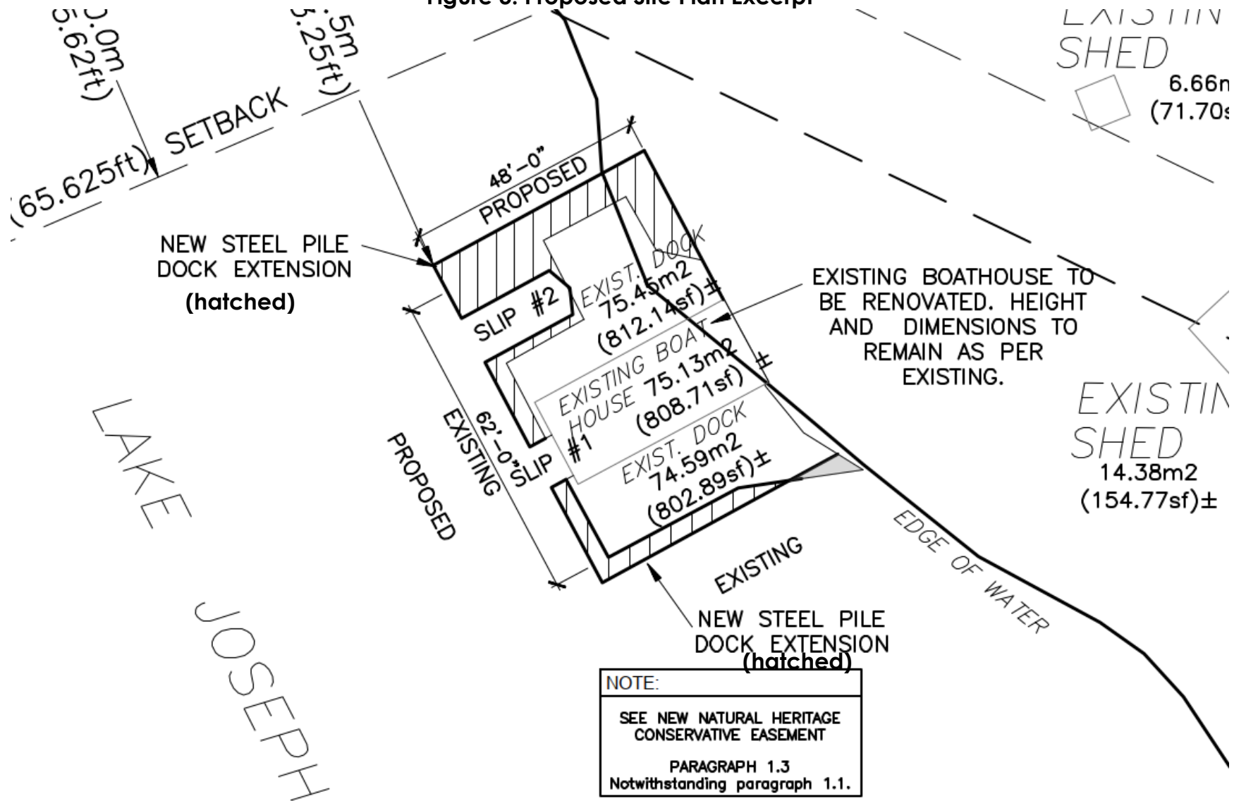
Figure 3: Proposed Site Plan Excerpt
